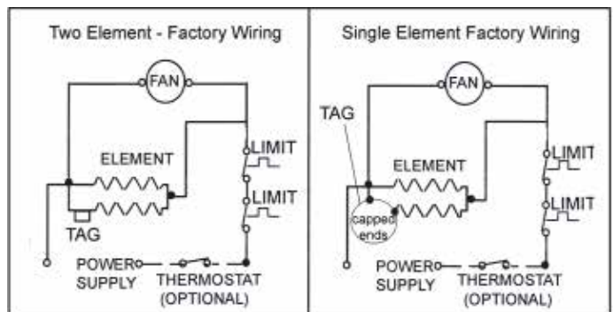
Wiring Diagram
